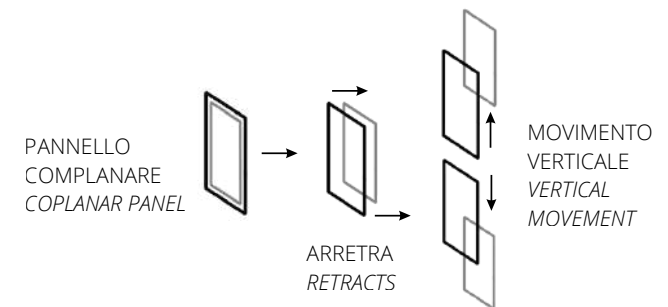
COPLANAR PANEL
