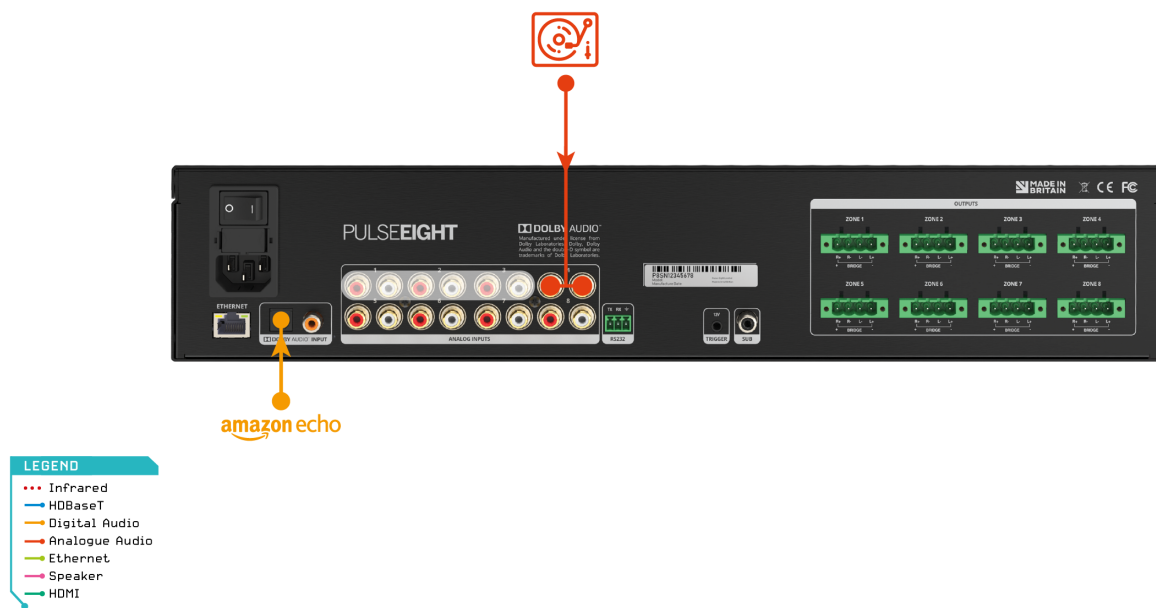
Figure 1: Connecting the audio input for 3 Zone Dolby Mode
