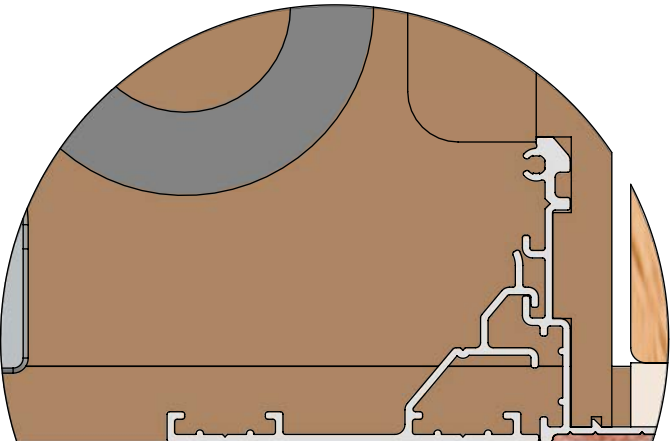
DETAIL E - 75mm FLAP - NO MDF SCALE 2 : 3
