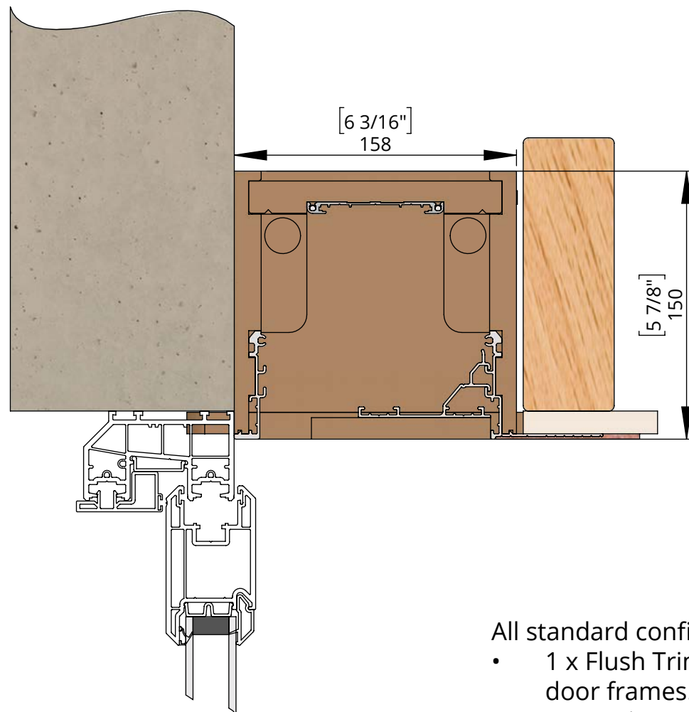
UCH-SINGLE-95 - SINGLE SHADE UPTO 95MM ROLLUP
