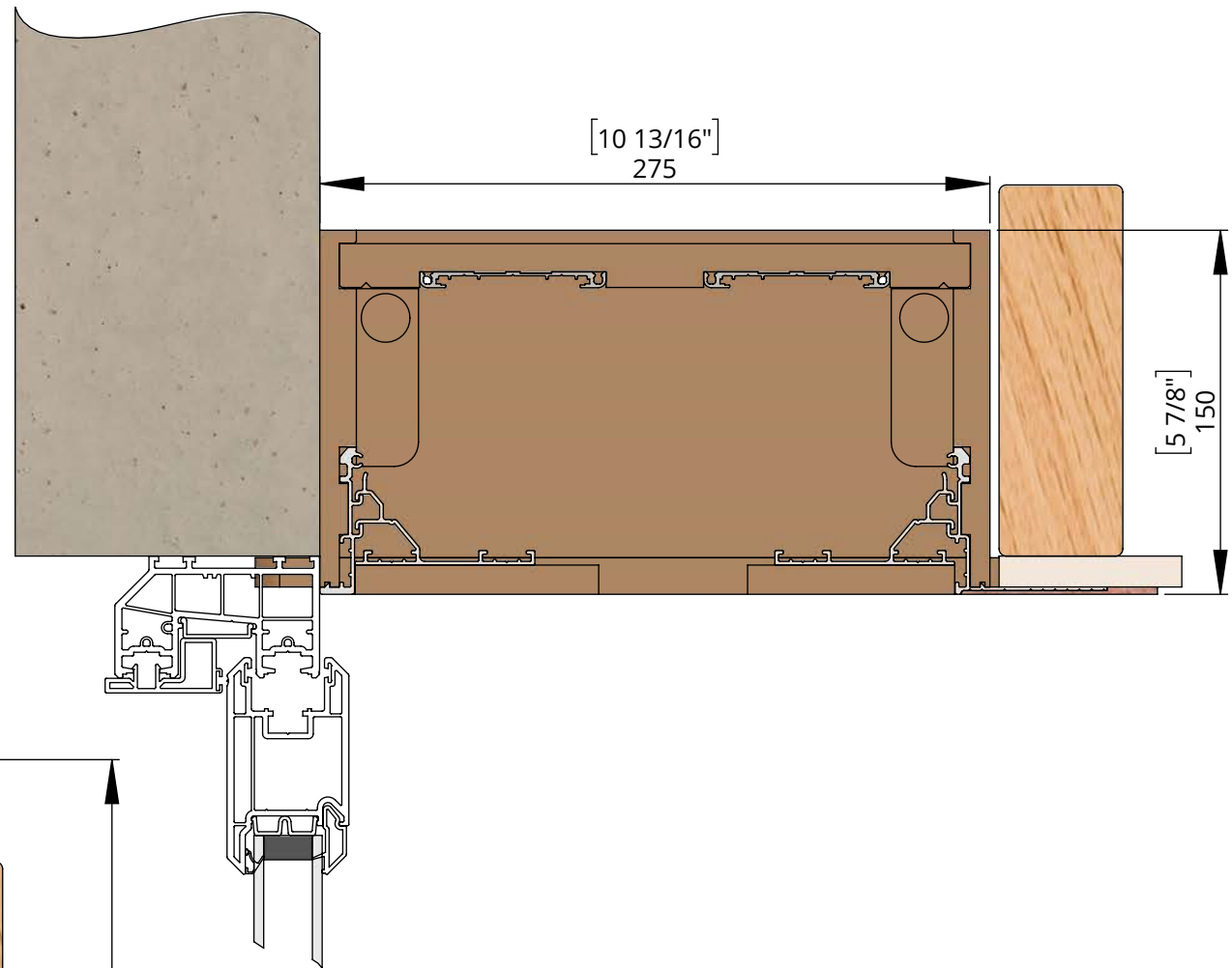
UCH-TWIN-75 - TWIN SHADE UPTO 75MM ROLLUP
