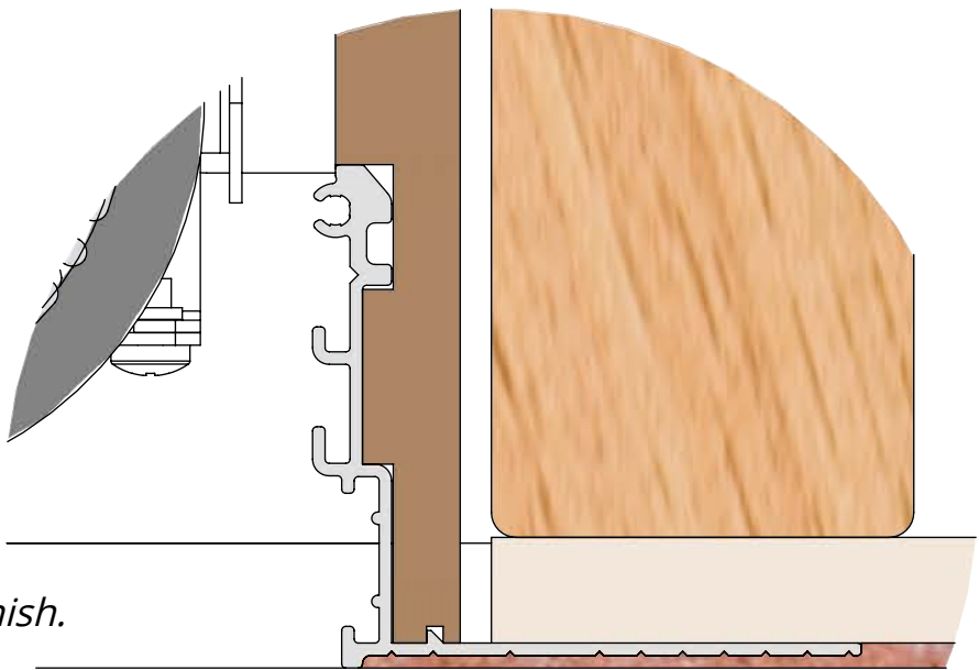
HORIZONTAL SKIM TRIM
