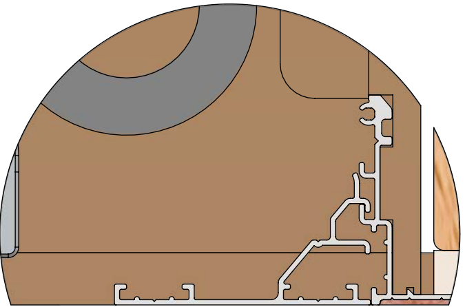
DETAIL C - 4" FLAP - NO MDF SCALE 2 : 3
