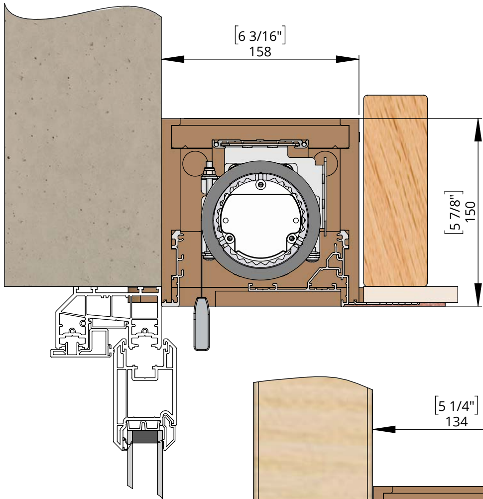
UCH-SINGLE-95 Single shade pocket for upto 95mm roll up shades, window side Flush Trim profile, room side Horizontal Skim Trim profile, UK spec 100mm Flap with 100mm deep 12mm thick MDF Flap material.
