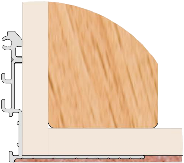
SPT - SHADE POCKET TRIM (Horizontal Skim Trim Used Standalone)
