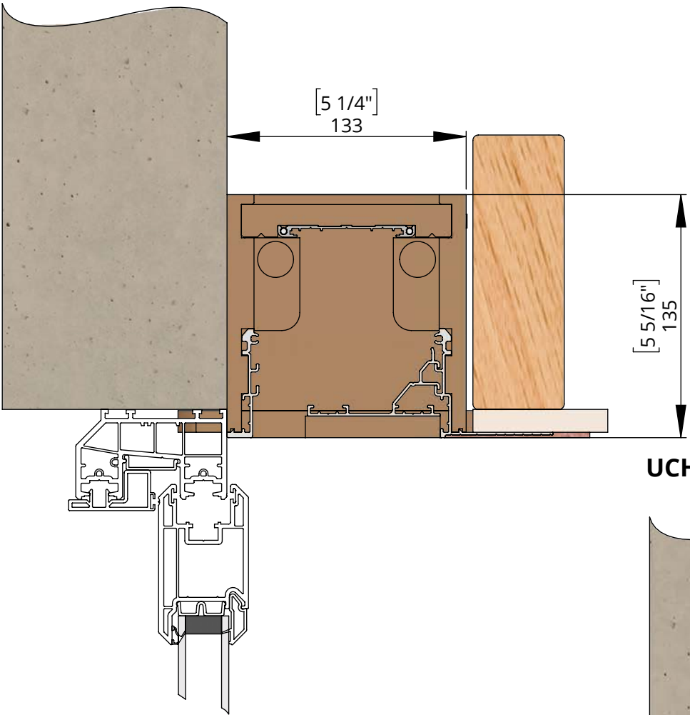
UCH-SINGLE-75 - SINGLE SHADE UPTO 75MM ROLLUP
