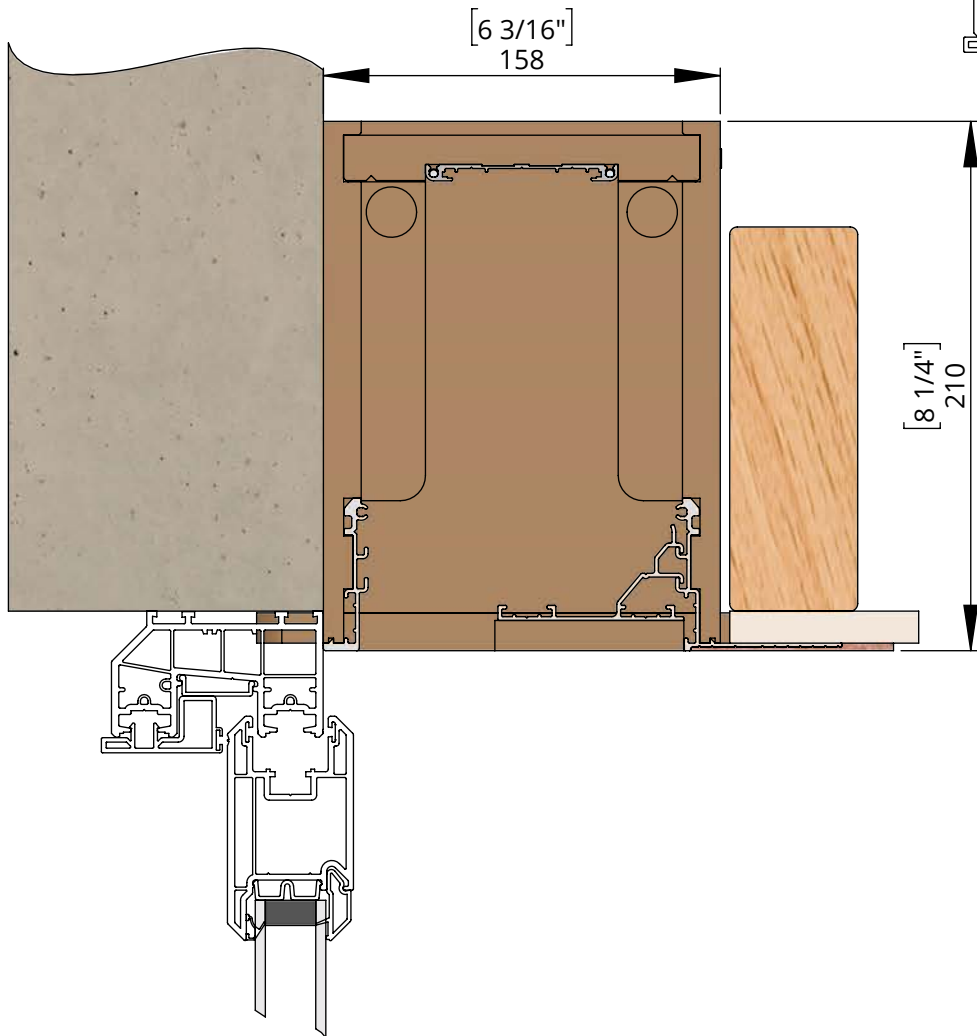
UCH-TWIN-75 - TWIN SHADE UPTO 75MM ROLLUP
