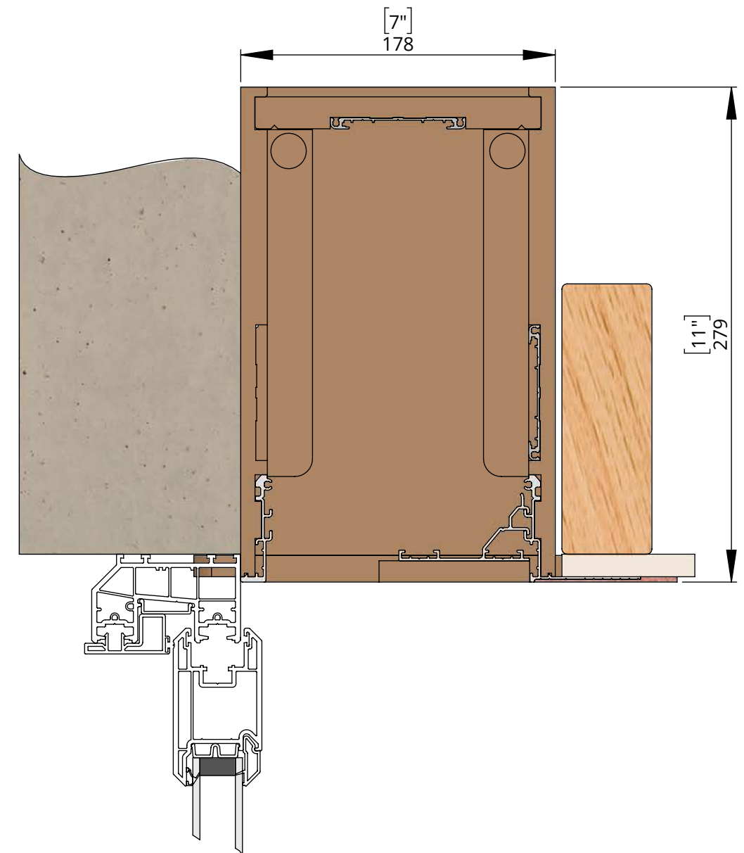
UCH-TWIN-95 - TWIN SHADE UPTO 95MM ROLLUP
