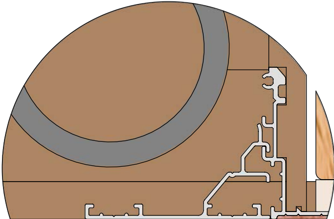
DETAIL D - 100mm FLAP - NO MDF SCALE 2 : 3
