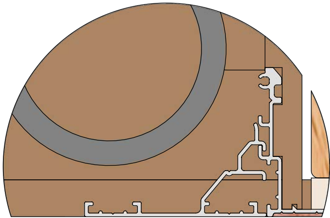
DETAIL B - 4" FLAP - NO MDF SCALE 2 : 3
