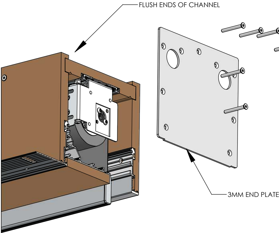
FLAT METAL END PLATE
