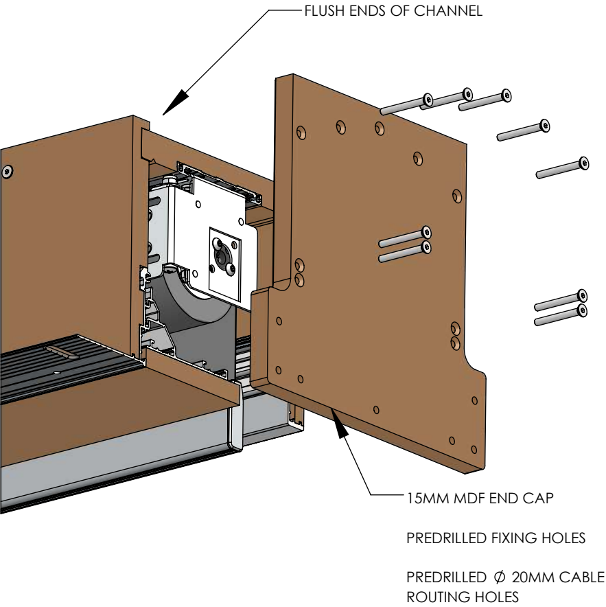
VERTICAL SKIM END PLATE
