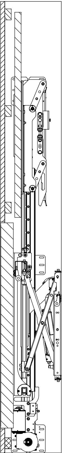
ADVANCE - OUT
