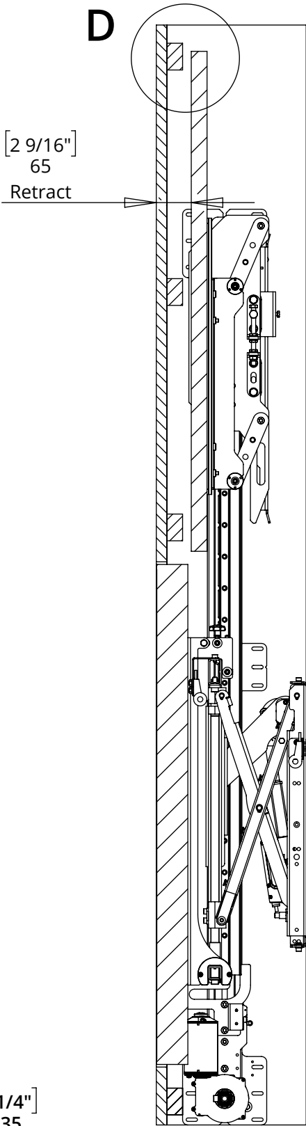
Screen - OUT
