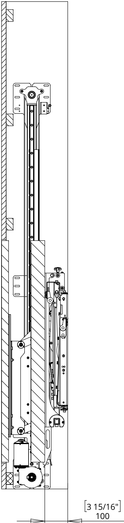
ADVANCE - IN
