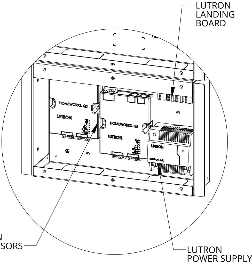
LCP PDPS - POWER SUPPLY ADD ON UNIT
